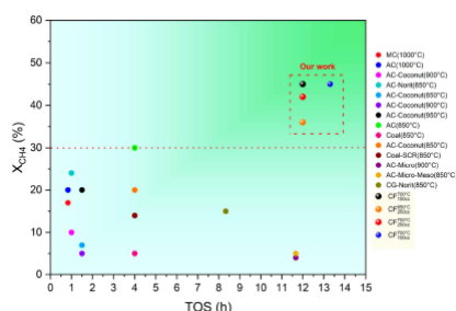
Figure 1. Comparison of CH 4 conversion under CH (literature) and IH (our work)
